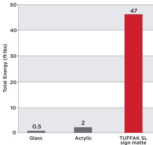
Impact Resistance*
