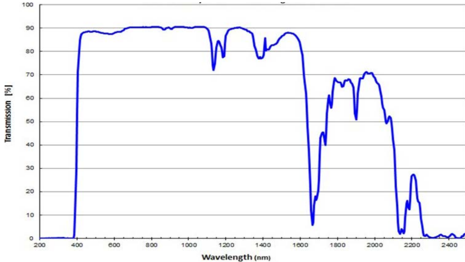
TUFFAK® Polycarbonate Sheet Light Transmission
