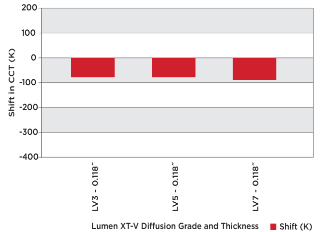
Correlated Color Temperature Shift for a 3000 K LED
